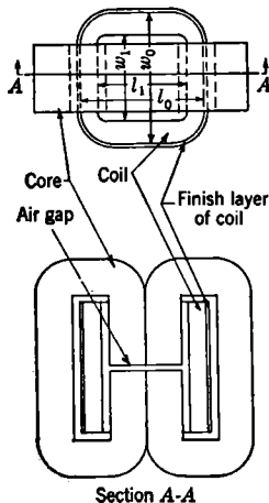
FIG. 9-11.—Sketch of d-c resonant-charging reactor.
